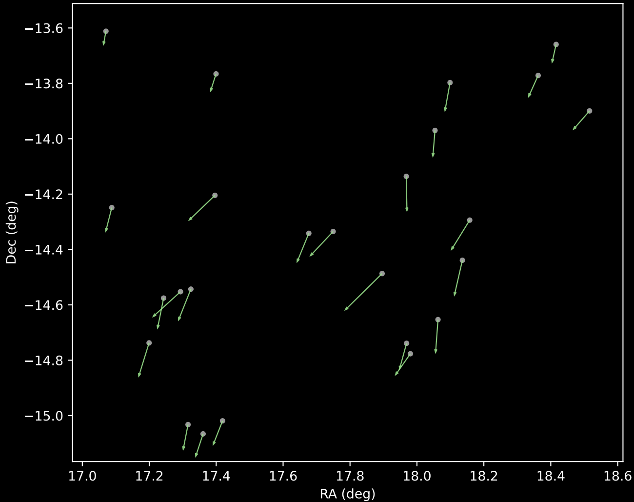
APOGEE DR17 Cluster 5 Proper Motion Vectors (n=25)
