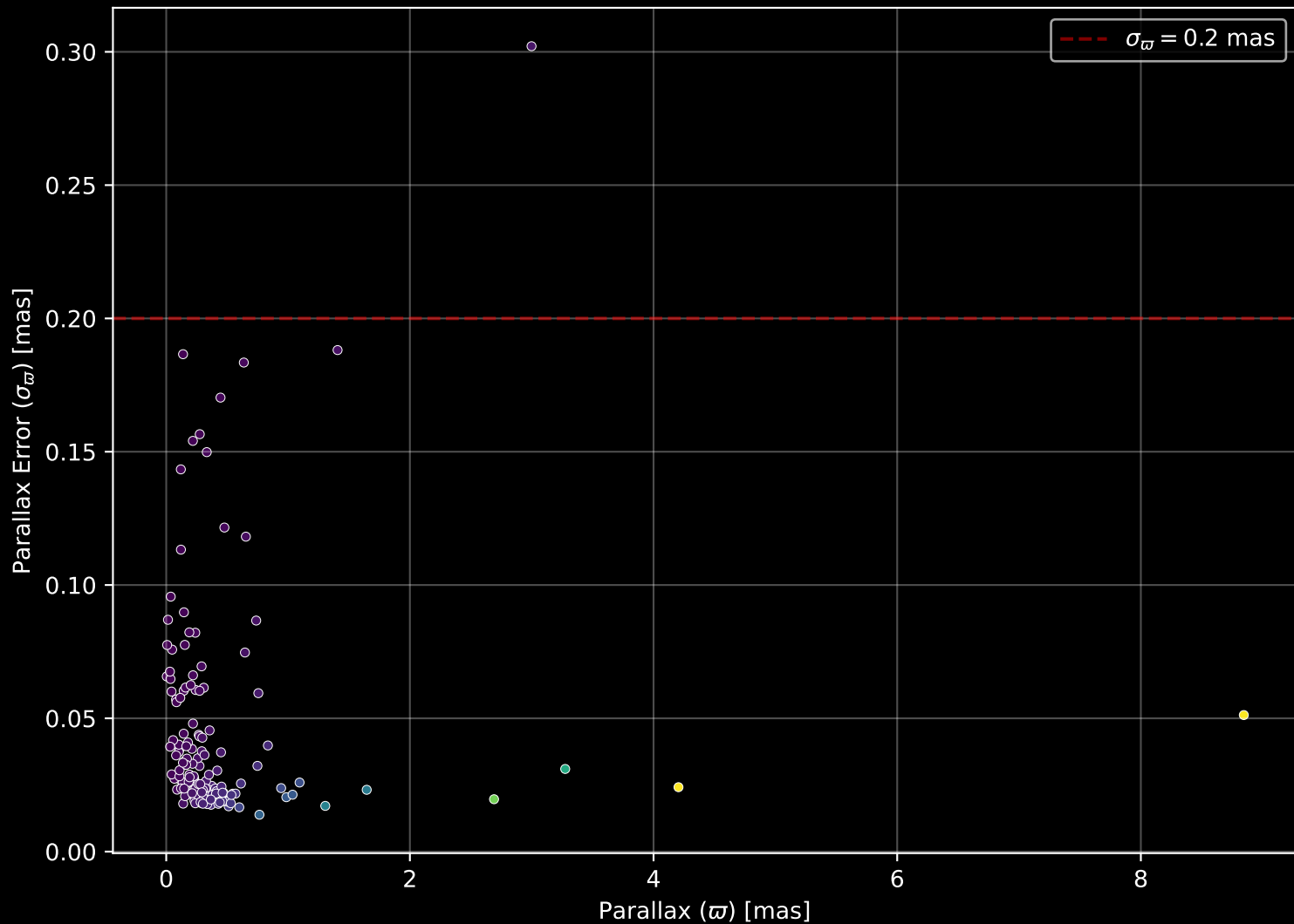
APOGEE DR17 Field: [018-02] Parallax Quality (n= 144)
