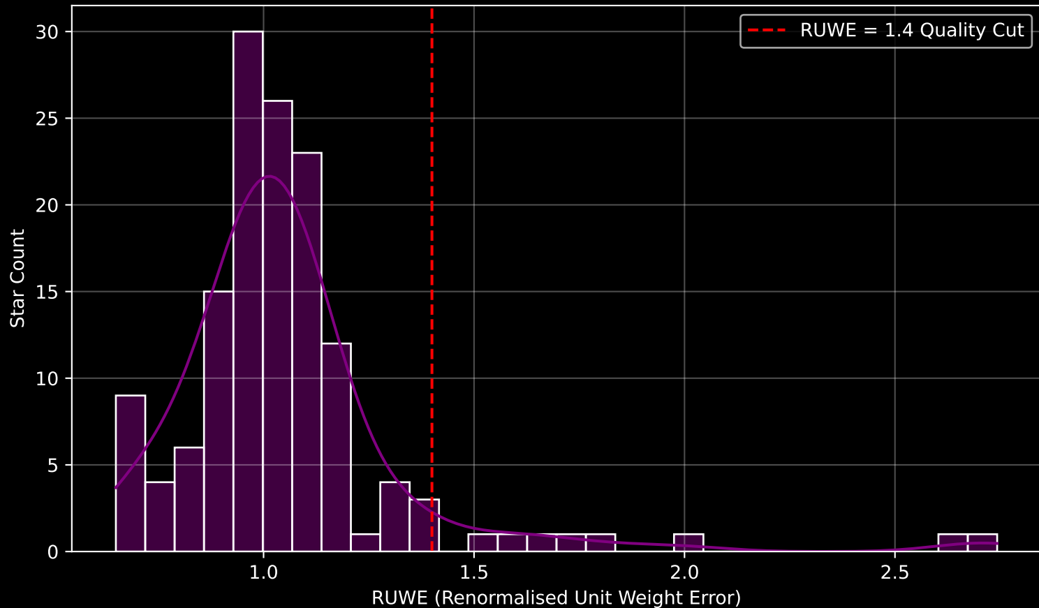
GAPOGEE DR17 Field [018-02] RUWE Distribution (n= 141)
