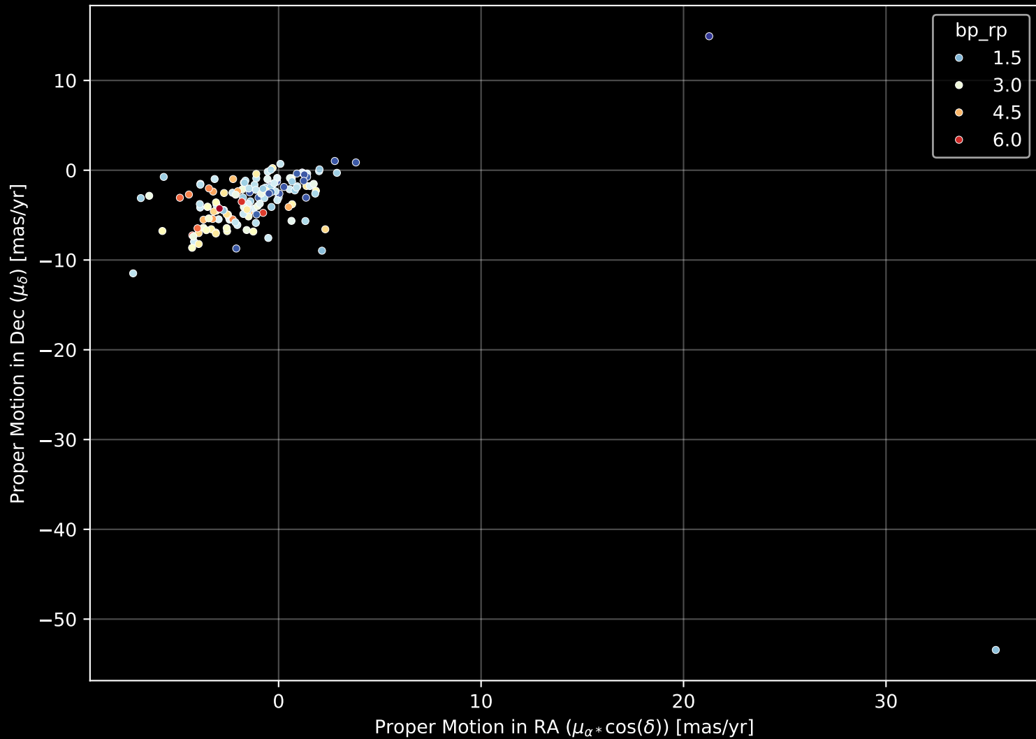
APOGEE DR17 Field: [018-02] Proper Motion Diagram (n= 144)
