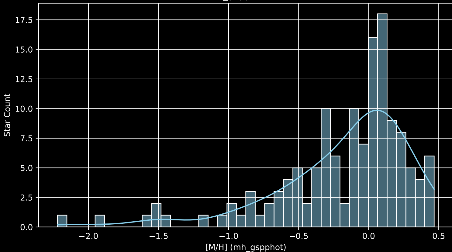
APOGEE DR17 Field: [018-02 [M/H] (mh_gspphot) (n= 137)
