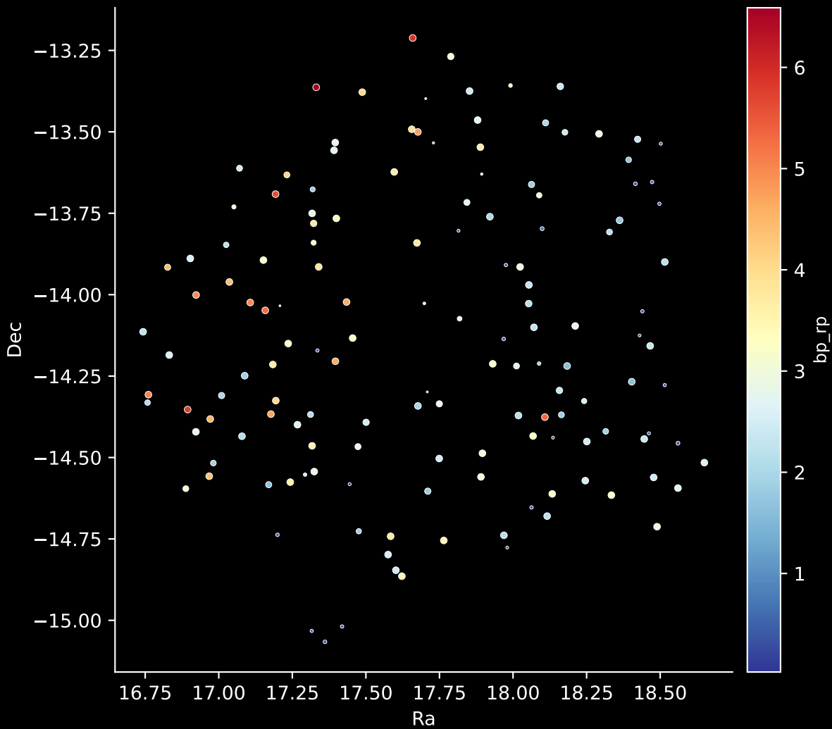
APOGEE DR17 Field: [018-02] Stars: 144
